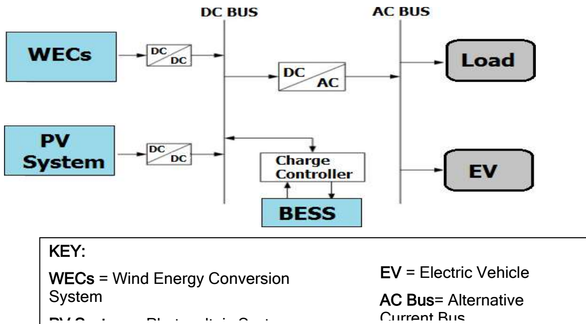
Figure 3.2 Hybrid system optimization
