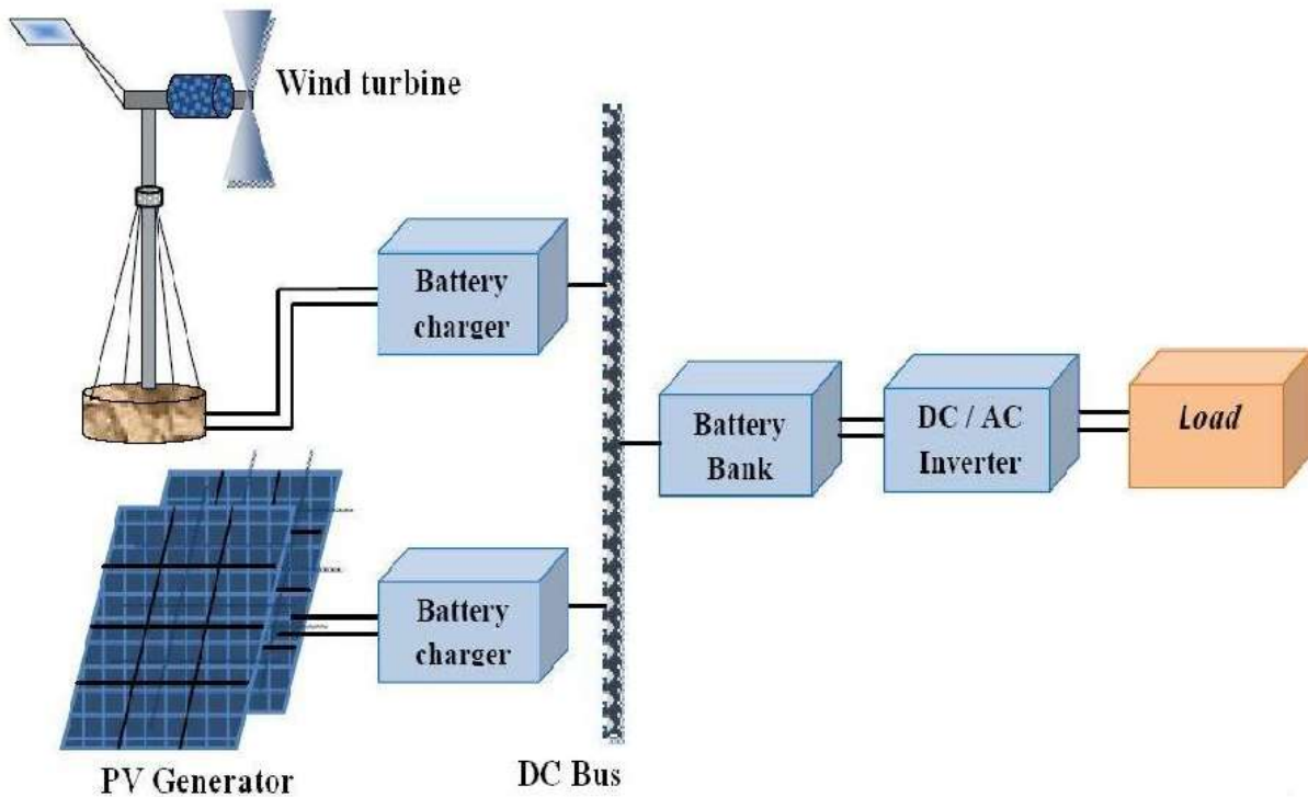
Fig. 1.1 HYBRID WIND/PV STANDLONE GENERATION SYSTEM
