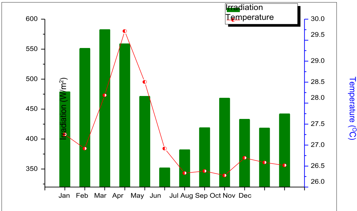
Figure 4.1 Global Horizontal Irradiation and Air Temperature at Central University of Kerala
