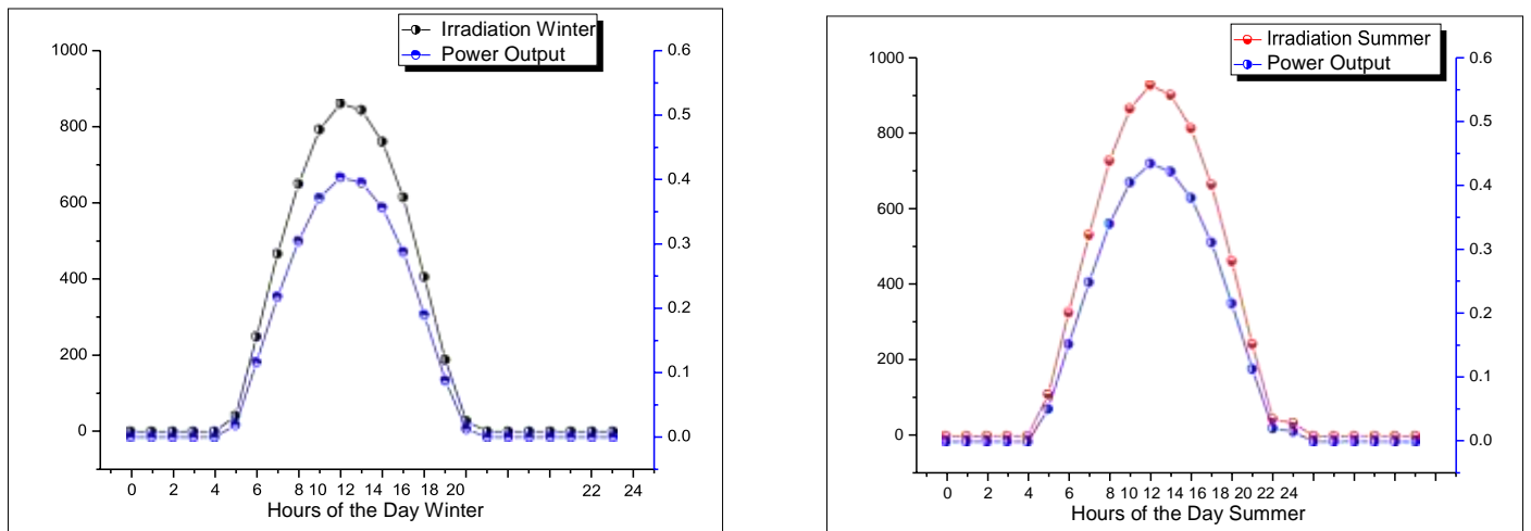
Figure 4.4 Diurnal irradiation and 600Wp performance at Central University of Kerala: a) Winter; b) Summer;
